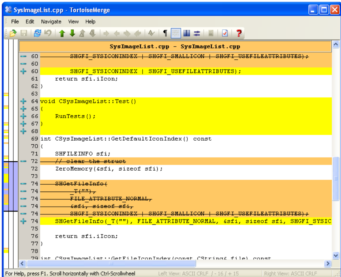
Figure 3.1. One Pane View
