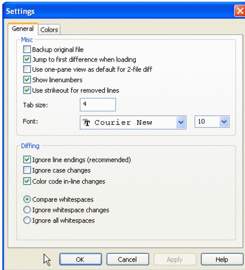
Figure 3.7. The Settings Main Page
