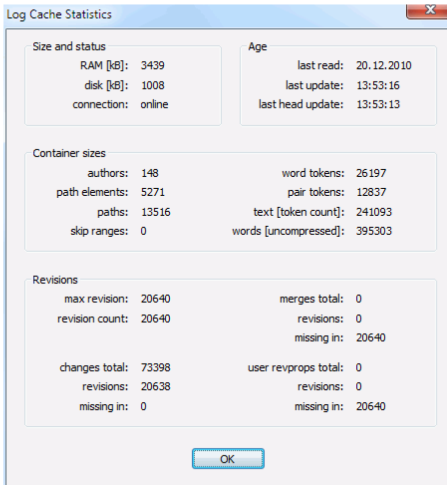
Figure 4.88. The Settings Dialog, Log Cache Statistics
