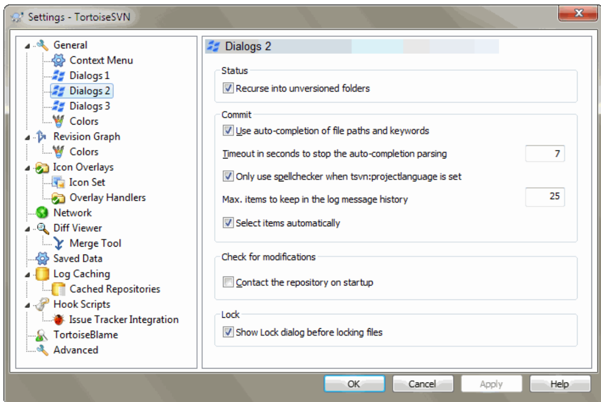
Figure 4.75. The Settings Dialog, Dialogs 2 Page
