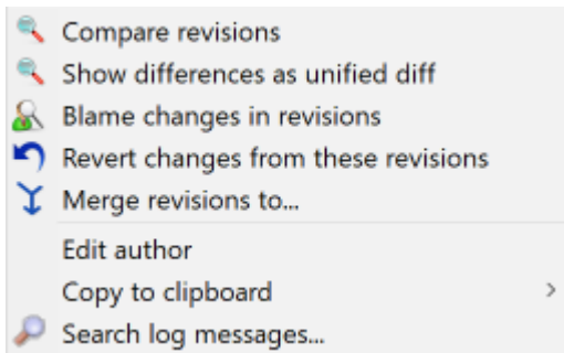
Figure 4.21. Top Pane Context Menu for 2 Selected Revisions
