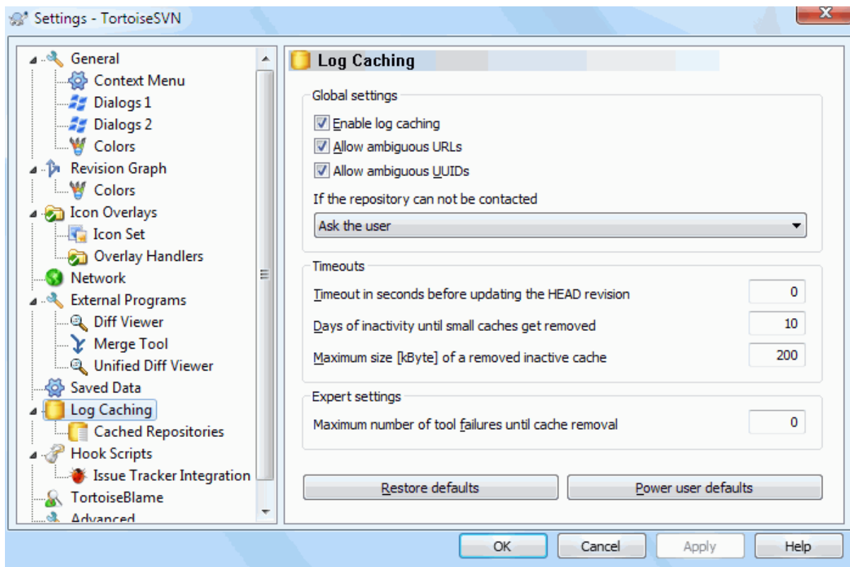
Figure 4.87. The Settings Dialog, Log Cache Page
