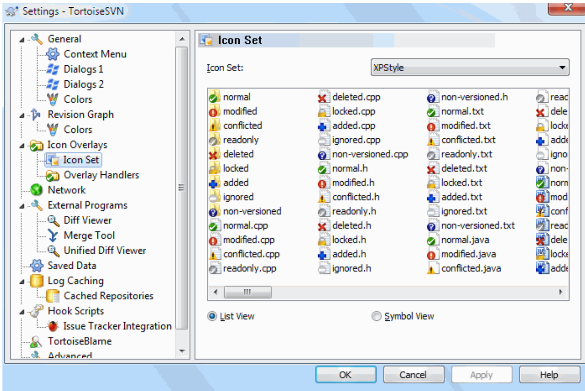
Figure 4.81. The Settings Dialog, Icon Set Page
