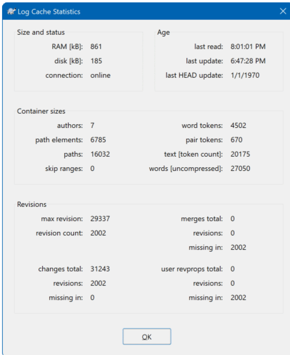
Gambar 4.88. The Settings Dialog, Log Cache Statistics
