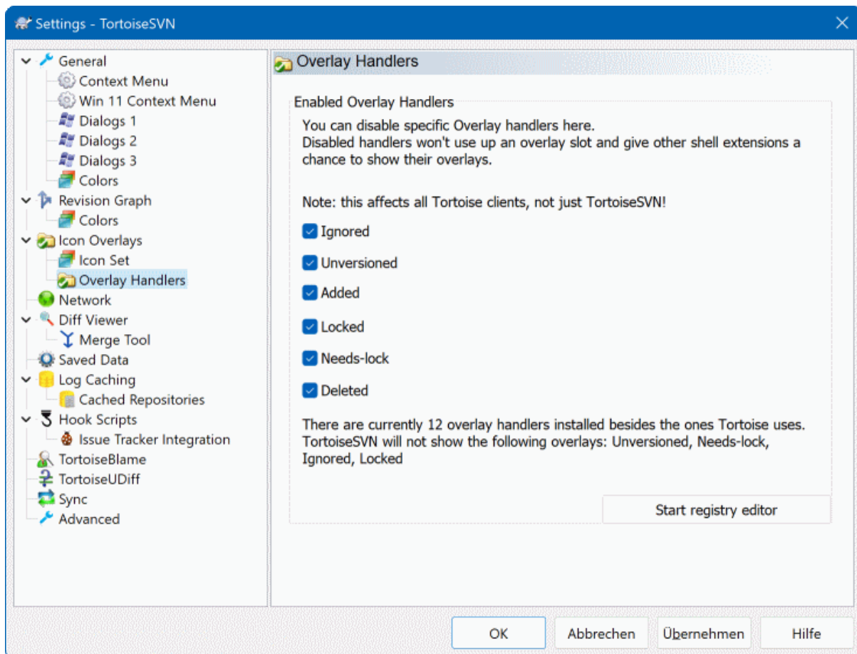
Gambar 4.82. The Settings Dialog, Icon Handlers Page
