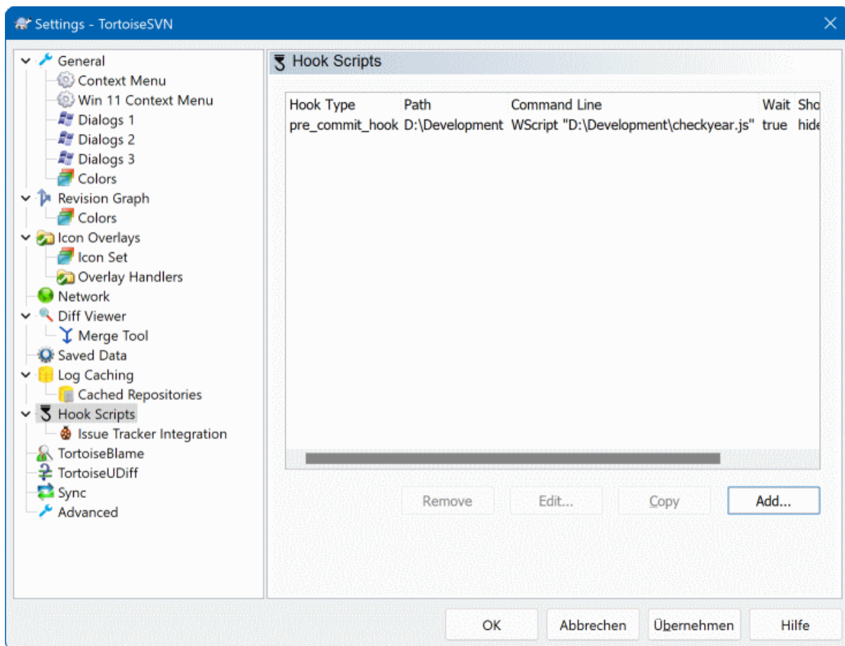
Gambar 4.89. Dialog Setting, Halaman Naskah Hook
