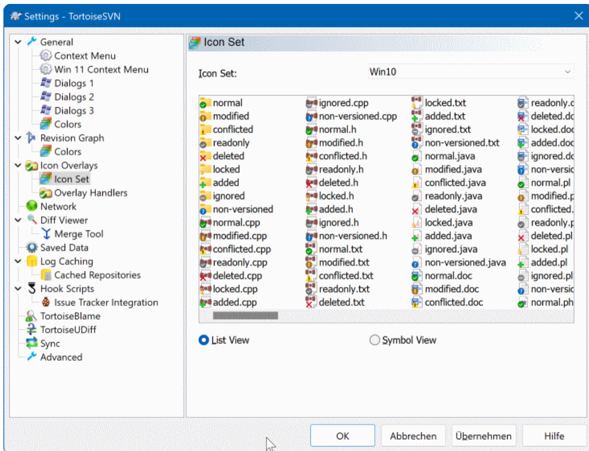
Gambar 4.81. HDialog Seting, Halaman Set Ikon
