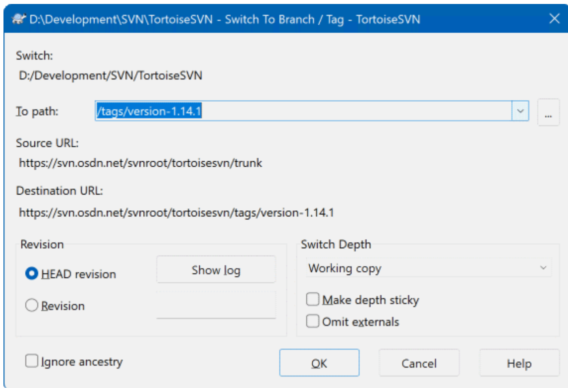
Gambar 4.55. Dialog Tukar
