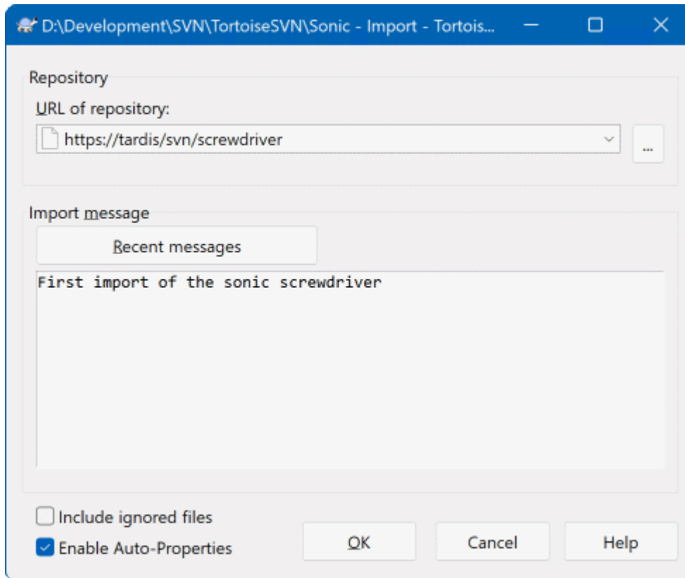
Gambar 4.6. Dialog Impor
