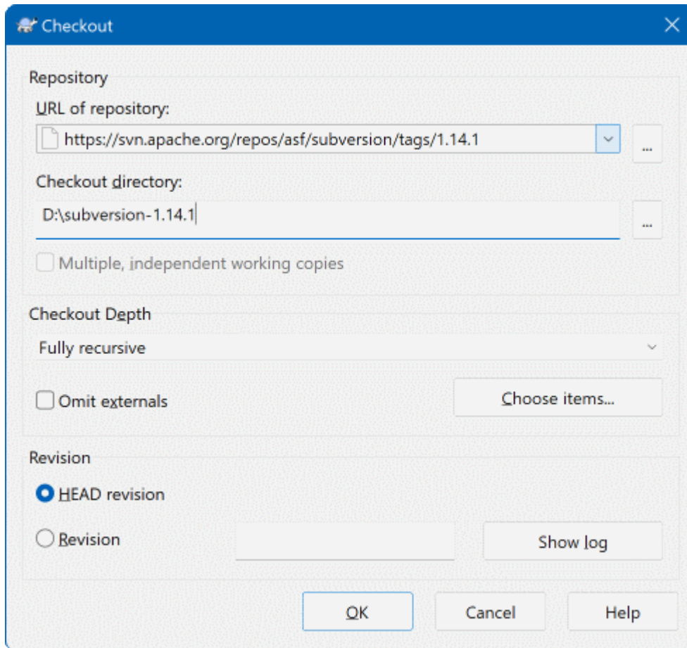
Gambar 4.7. Dialog Checkout
