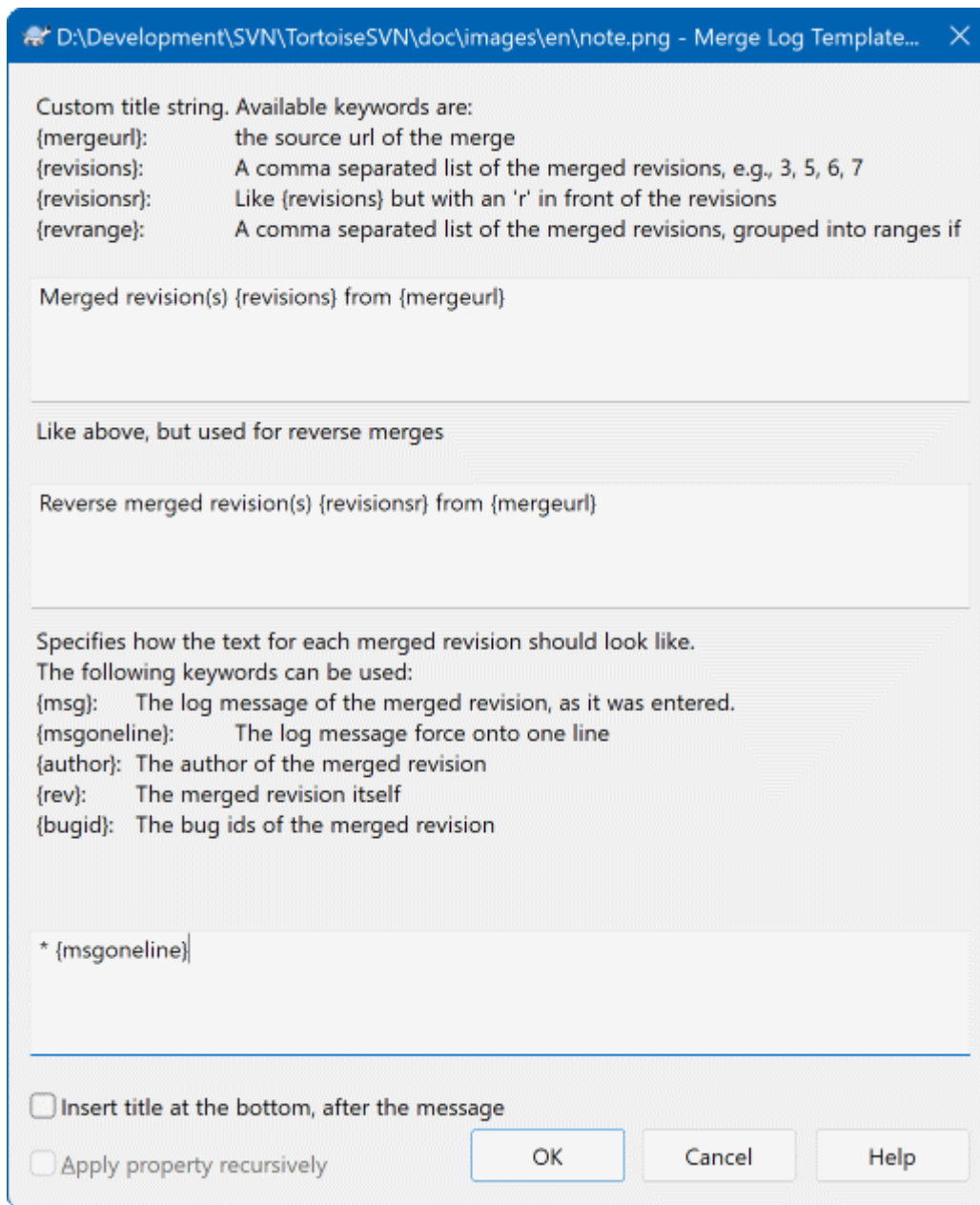
Gambar 4.53. Property dialog merge log message templates
