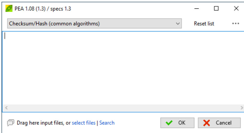
Image 29: PeaUtils
